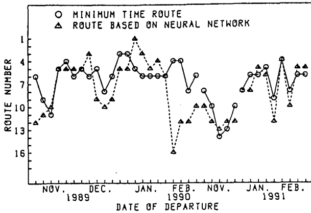
Fig.8 Comparison of route numbers of the routes based on the WRNN with those of the minimum time routes
