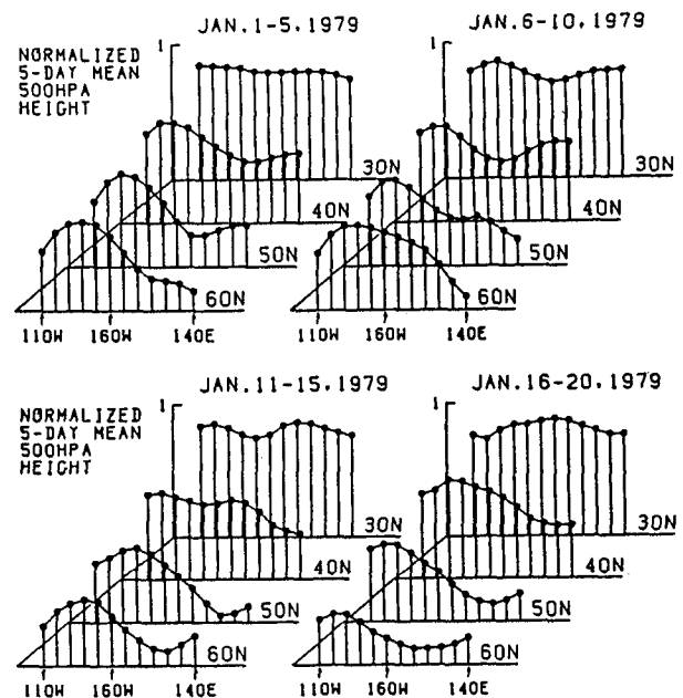
Fig.3 Example of input signals to the WRNN (Jan.1-20, 1979)
