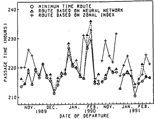
Fig.9 Comparison of passage times on the routes based on the WRNN with those based on the zonal index and those of the minimum time routes
