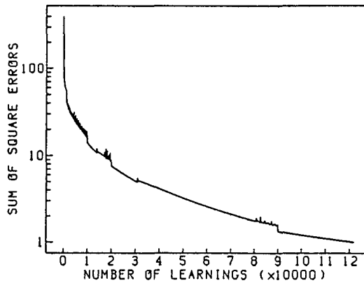
Fig.5 Change of the error of output signals during the learning process
