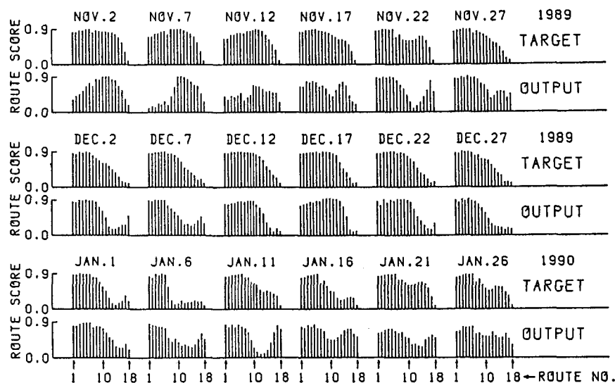
Fig.7 Comparison of the output signals from the trained WRNN with the target signals
