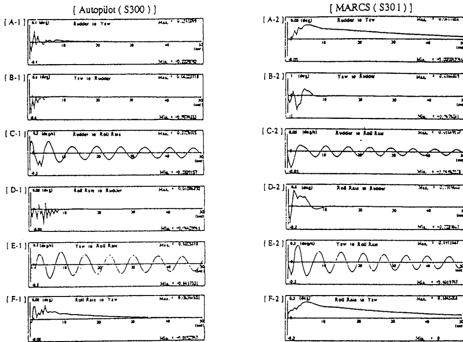
[A] , [B] Between Rudder and Yaw Deviation [C] , [D] Between Rudder and Roll Rate [E] , [F] Between Yaw Deviation and Roll Rate
