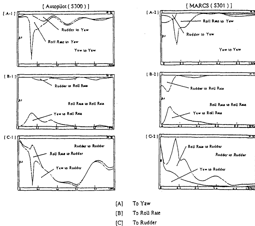
Fig. 5 Noise contribution function of the conventional autopilot and the MARCS
